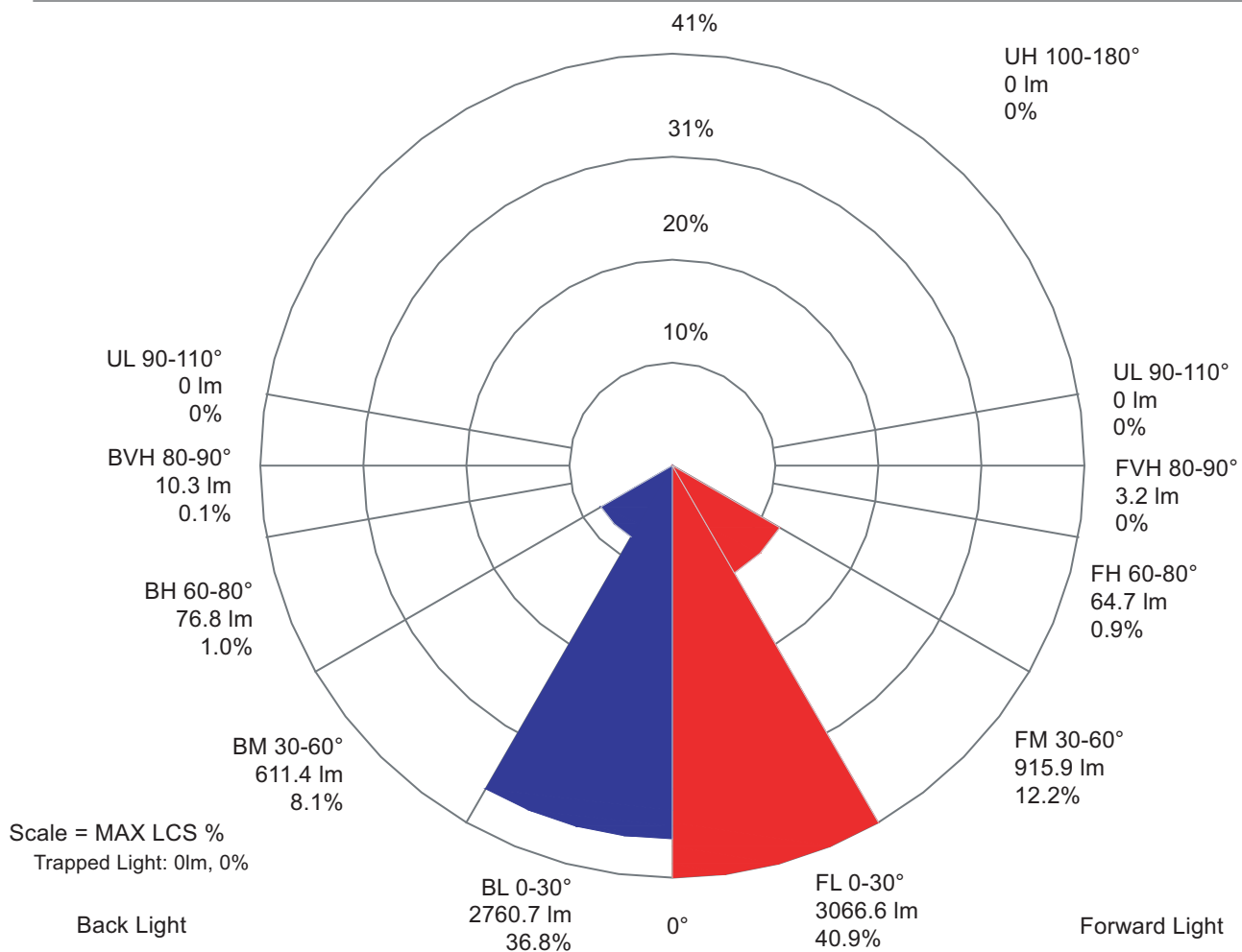
LCS graph
