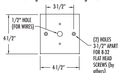
Mounting Plate size & mounting holes
