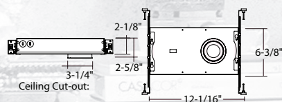
LSHLD2 2.5" Super-Shallow Frame New Construc- tion For LR2573 & LRX2573 (Round)
