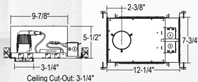
LHLD25IC-FRM/LHQLD25IC-FRM New Construction Insulation Contact Frame, Round or Square, For LRLD2573, LRXLD2573, LRLDQ2573 & LRXLDQ2573 (Round Shown)
