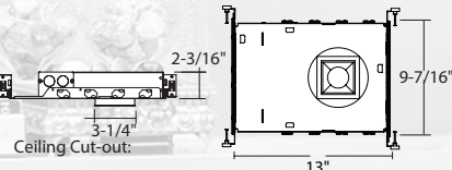
LSHQLD2 2.5" Super-Shallow Frame New Construction For LRQ2573 & LRXQ2573 (Square)
