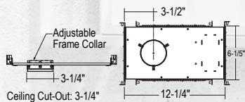
LHLD25-FRM/LHQLD25-FRM New Construction Frame, Round or Square For LRLD2573, LRXLD2573, LRLDQ2573 & LRXLDQ2573 (Round Shown)
