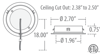
► LK136LED | Recessed Mount
