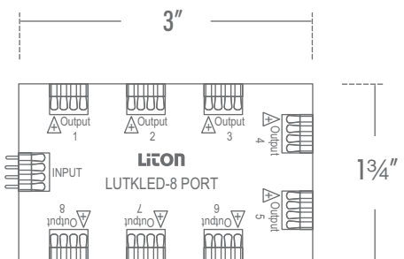
LUTKLED-PX8 8-Port Power Hub (LUTKLED-PH40 Included)
